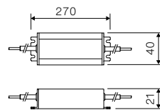
71/LDT9624 Voltage source 120-240Vac/24V 96W. Independent use.
